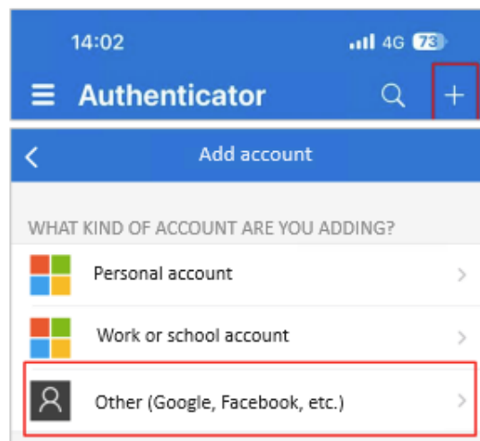
Create key
